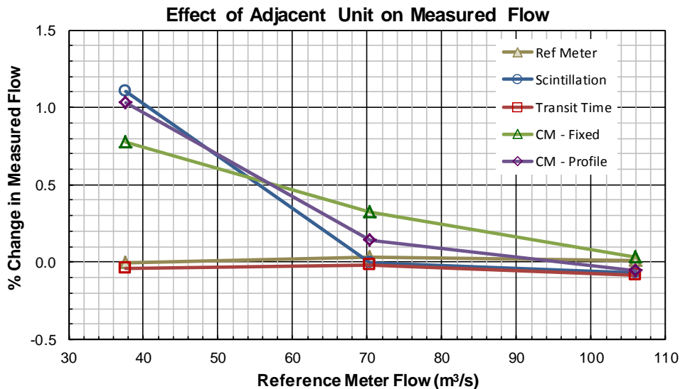
Figure 8 Effect of Adjacent Unit Operation
