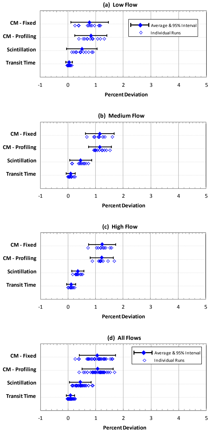
Figures 6(a) – 6(d) Plot of results relative to reference flowmeter
