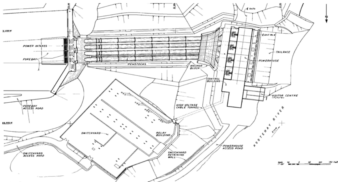
Figure 1 Plan View of Kootenay Canal Generating Station
