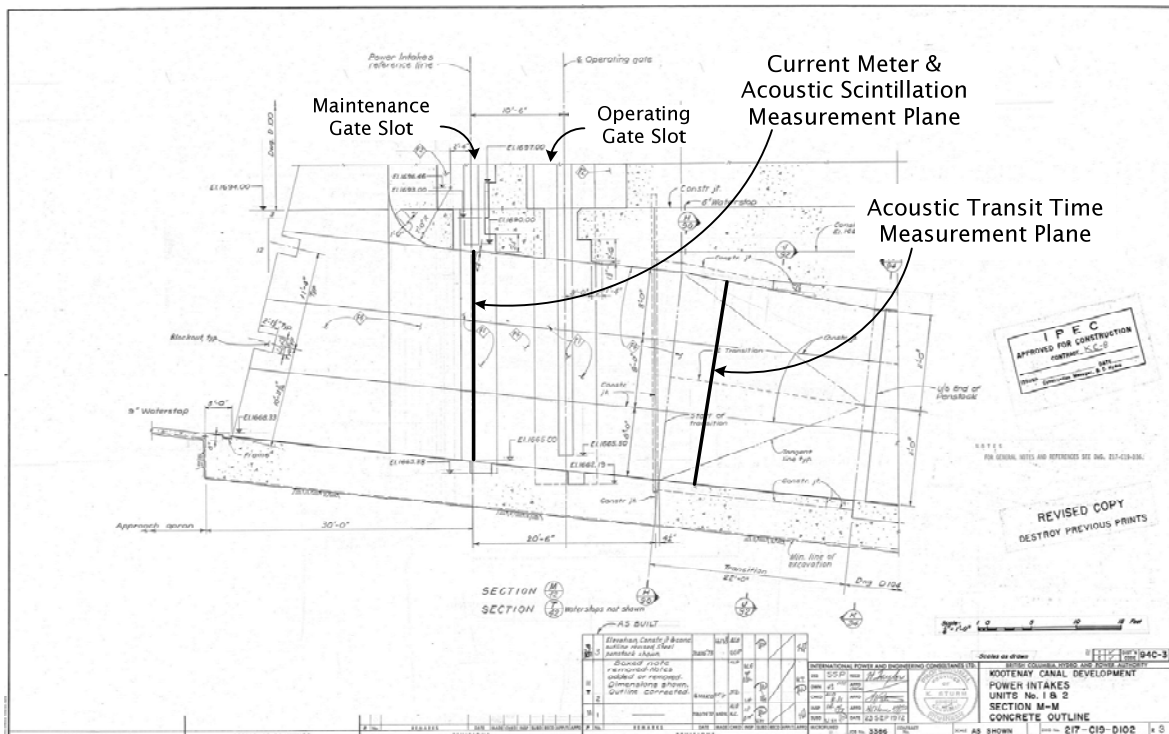
Figure 2 Location of Intake Flow Measurements
