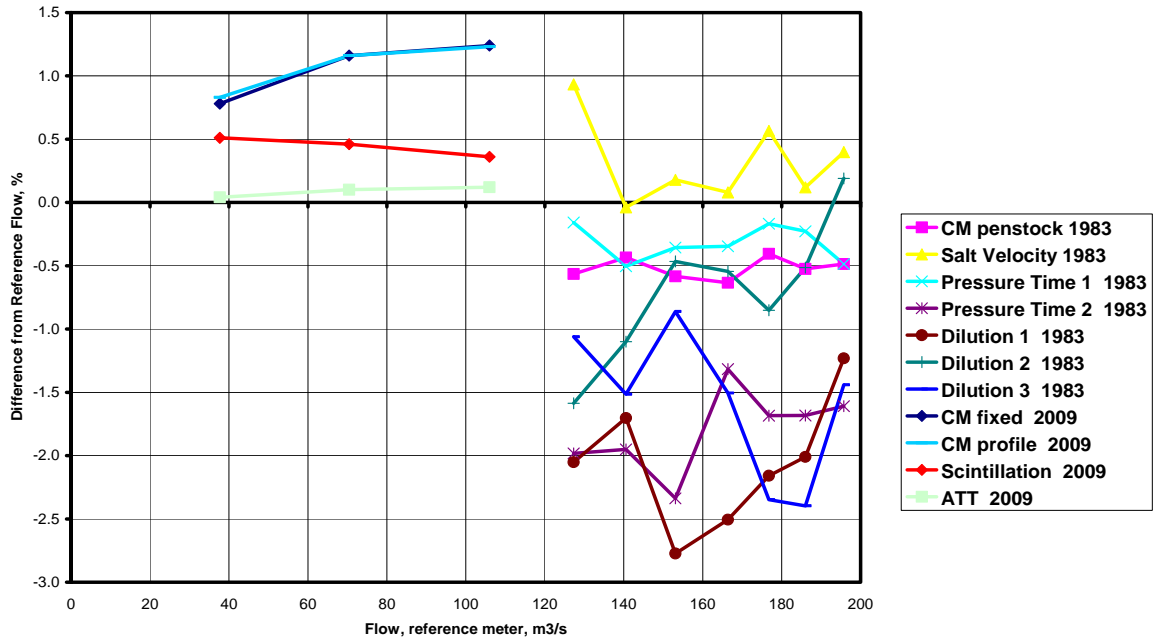
Figure 9 – Comparison of all data between 2009 and 1983
