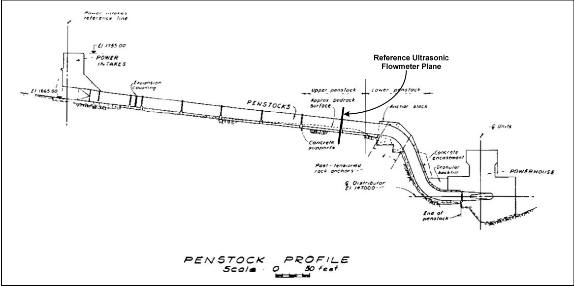
Figure 3 Location of Reference Flowmeter
