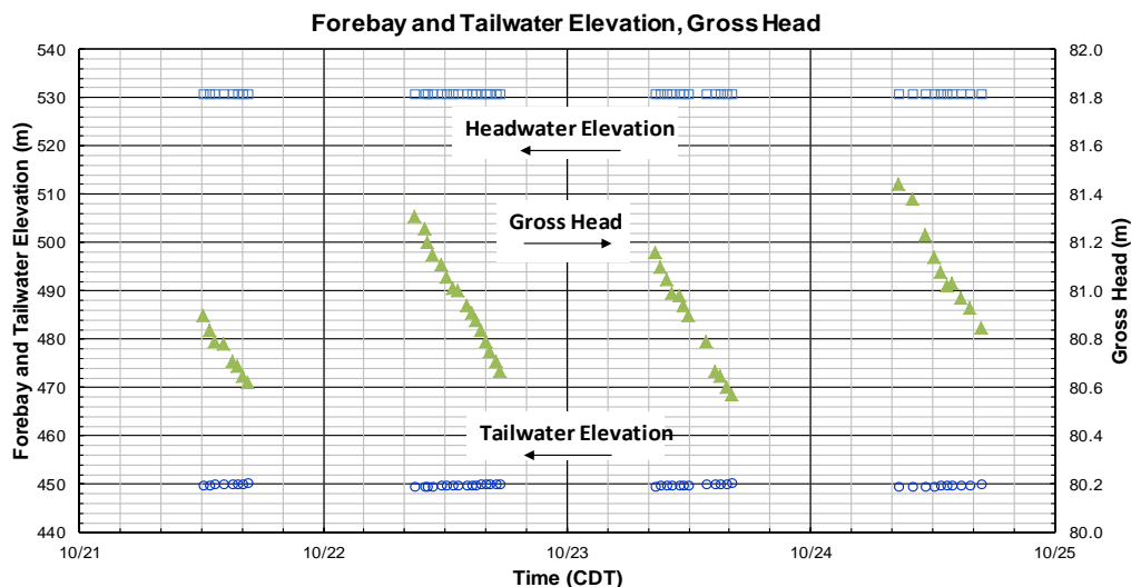
Figure 5 Variation in Head During the Test Program
