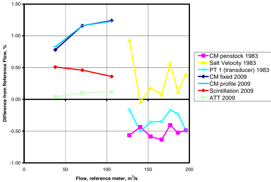
Figure 10 Comparison of commonly-used methods only
