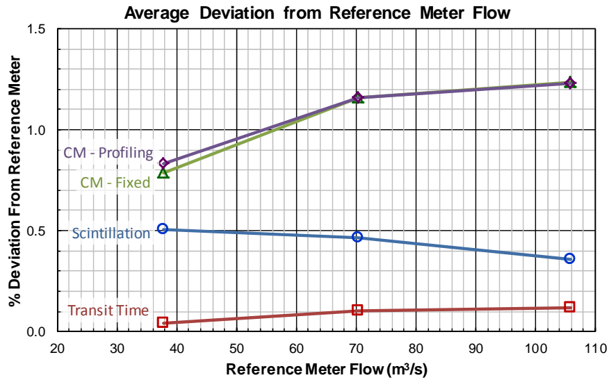
Figure 7 Average Deviation from Reference Meter Flowrate
